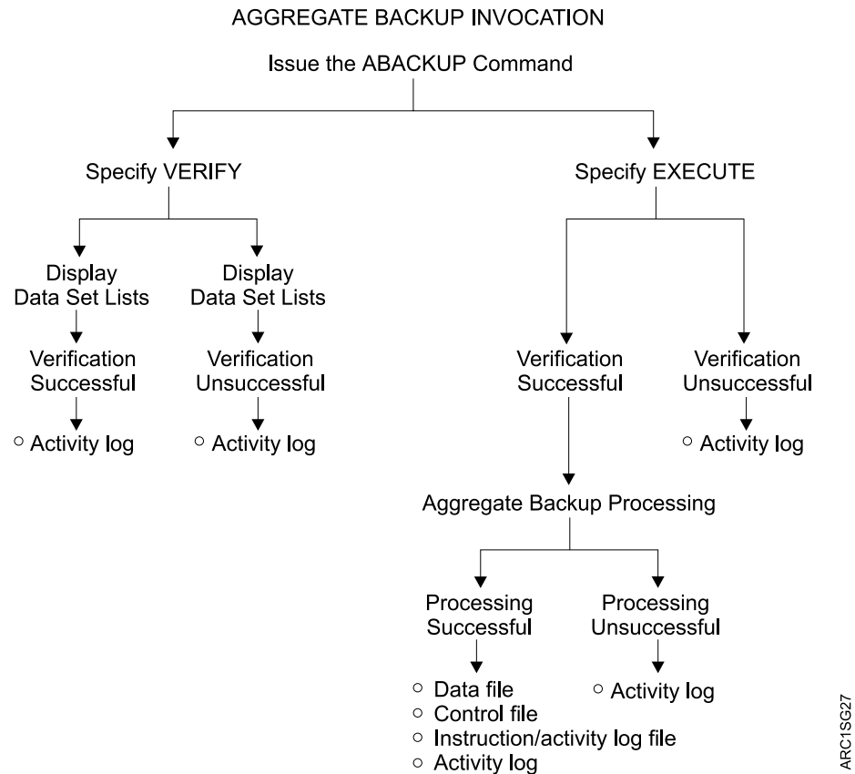
Figure 41. Aggregate Backup Invocation
