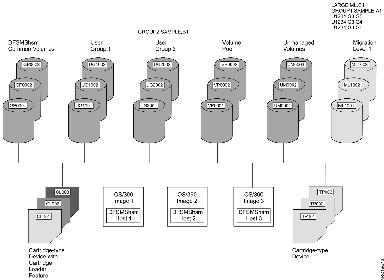
Figure 21. Example System for Non-SMS-Managed Volumes after Primary Volume Management Pass 2
